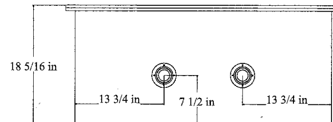
Discharge End View
