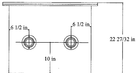
Discharge End
