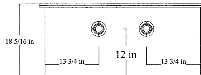
Inlet End
