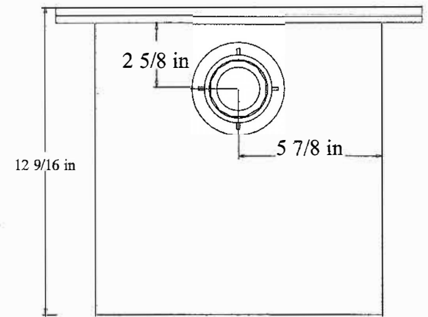
Discharge View
