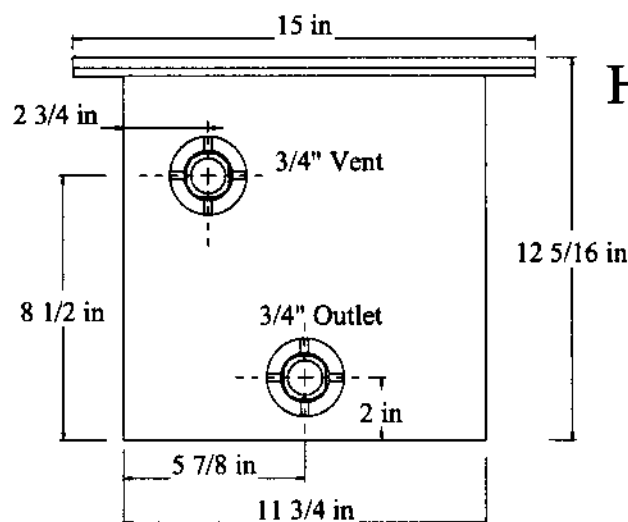
Outlet End View
